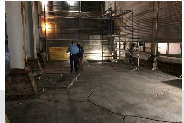
Figure 1 Cracks in the Concrete Basin Floor After Removal of the Tile Liner
